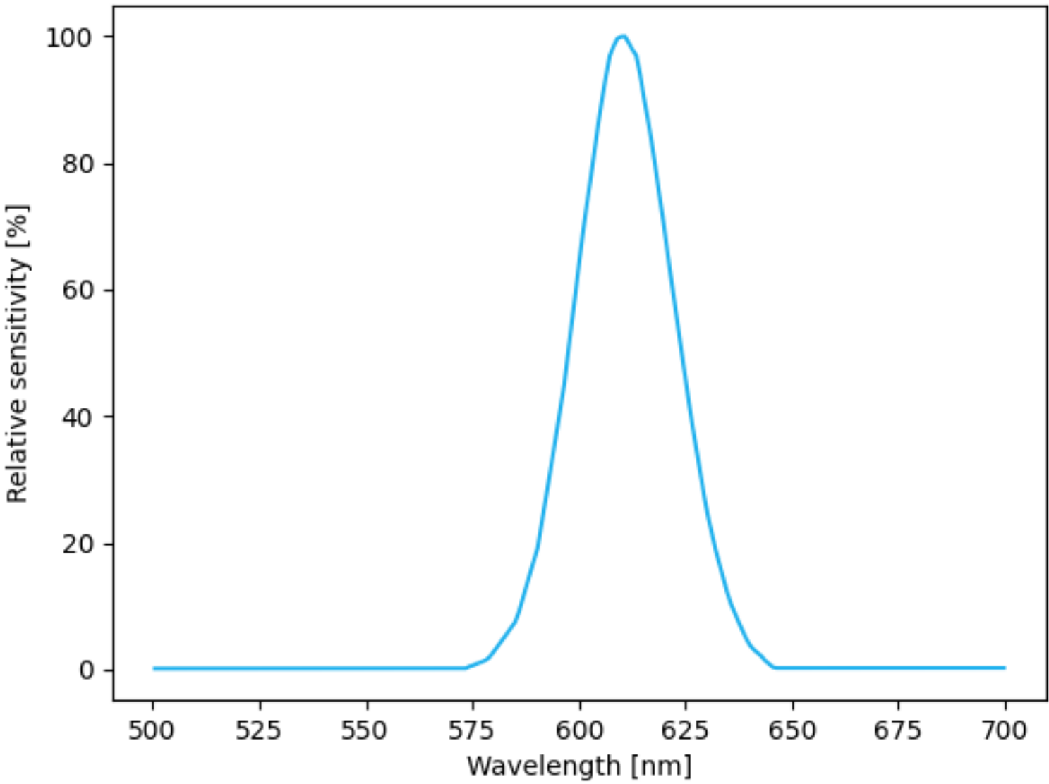
Sensor head spectral response
