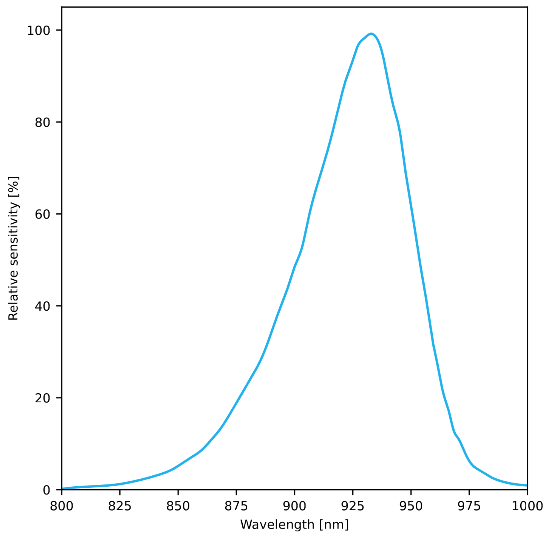
Sensor head spectral response
